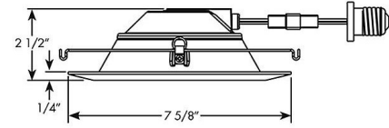
Height: 2 1/2" Width: 7 5/8"
